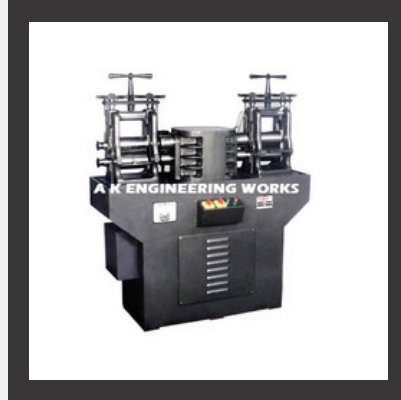
Double Head Wire & Sheet Rolling Mill
